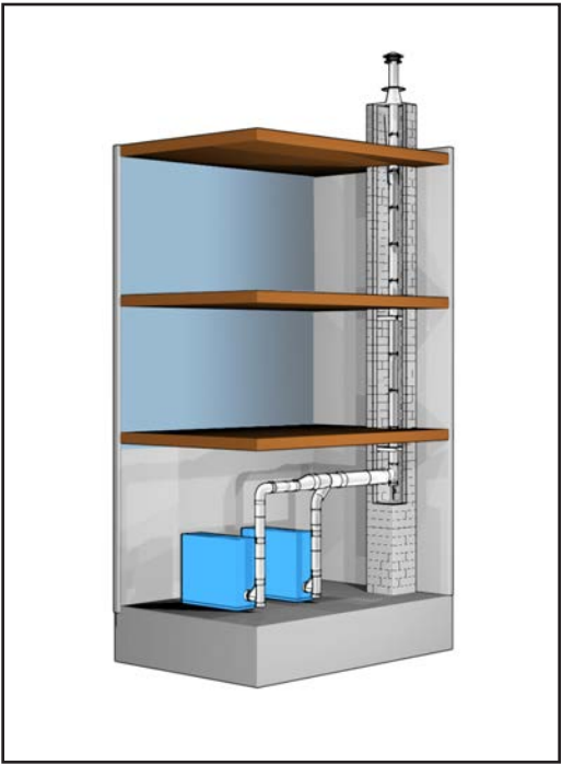
COMMERCIAL BOILER MASONRY CHIMNEY LINER
