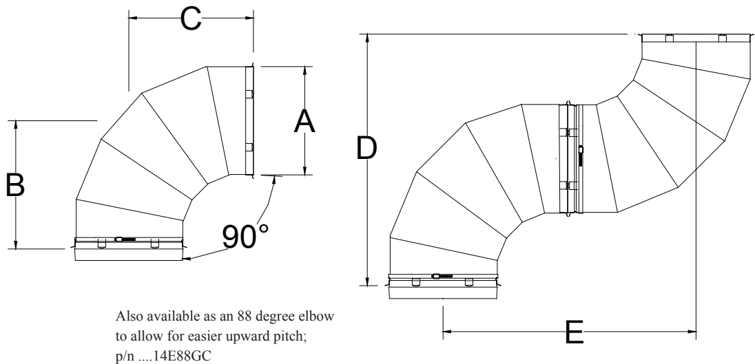
90° Elbow
